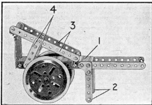
Fig. 2. A simple luggage truck.
