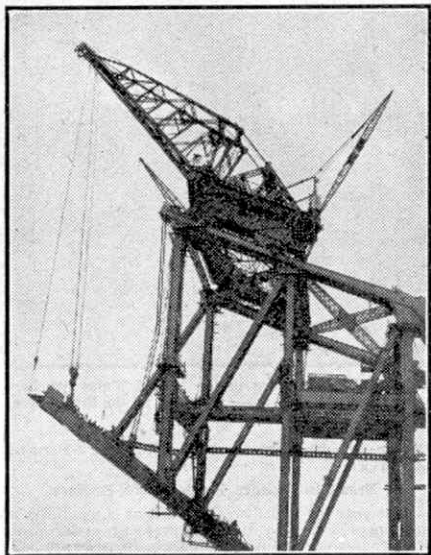
A closer view of one of the Creepers at work on the Sydney Bridge.
