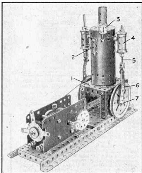
Fig. 1. A model vertical steam engine and boiler.
