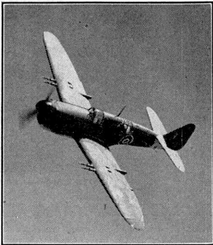
Fairley "Firefly," the first specially-designed cannon-armed British fleet fighter.
