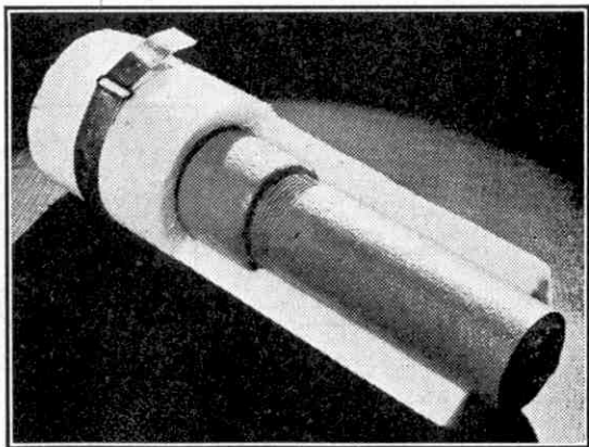
An example of Fibreglass wool used for lagging steam pipes. This picture shows how a rigid section of Fibreglass can be shaped to fit snugly around a junction between two lengths of piping.
