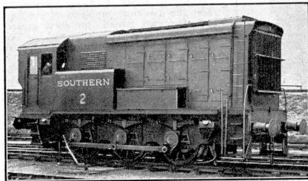
Southern Railway "English Electric" Diesel Locomotive.
