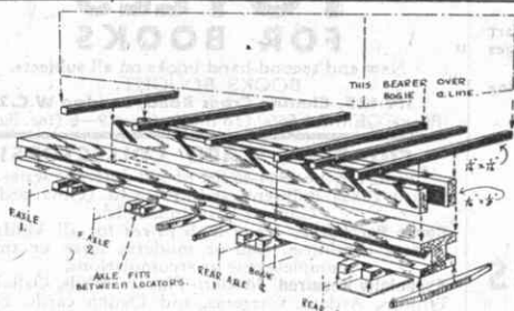
Exploded drawing showing undergear of a typical Wilson lorry.
