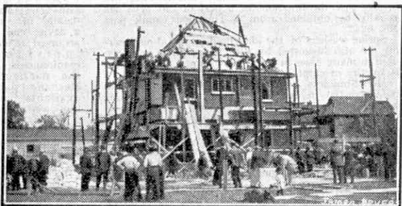
A house built in 17 hrs., as described on this page.
