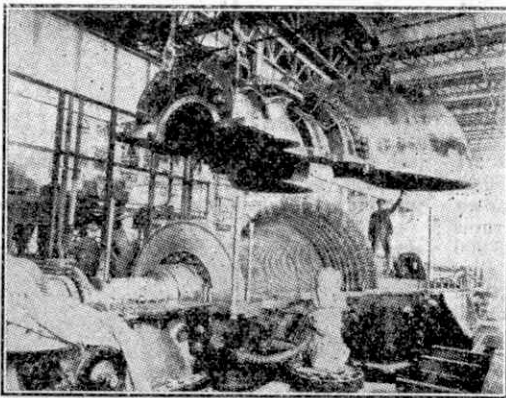
A 50,000 kW. Parsons Turbo-Alternator under erection.
