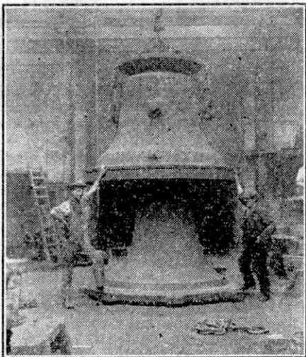
Cope and core, two parts of the mould for a bell.
