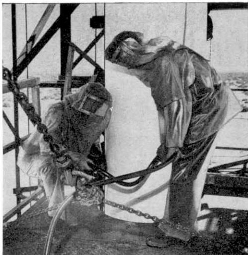
Protective clothing used while loading hydrogen peroxide into a Viking rocket. Illustration by courtesy of the Martin Co.
