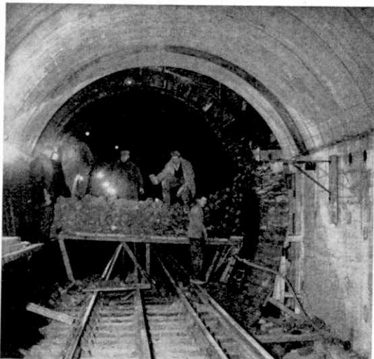
Renewing an old tunnel near Swiss Cottage on the Metropolitan Line. The section of old brickwork that has been broken down lies on the working stage ready for removal.
