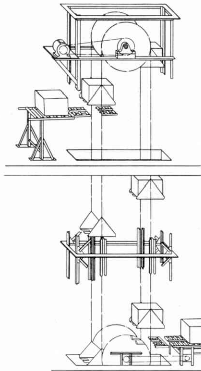
Fig. 2. A line drawing showing the general arrangement and principal features of The VertiVeyor passing through a floor of a building.
