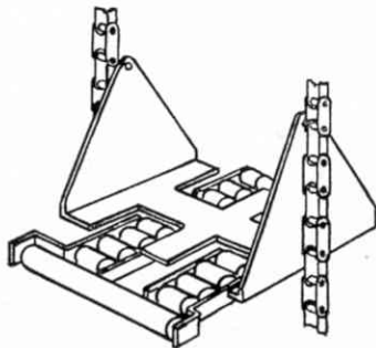
Fig. 4. A load carrier passing through a "pick-up" grid, which consists of fingers fitted with rollers. The feed-out grid is similar but is inclined slightly so that the loads run clear.
