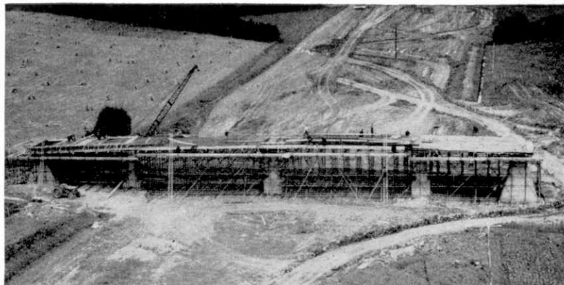
A four-span overbridge under construction.
