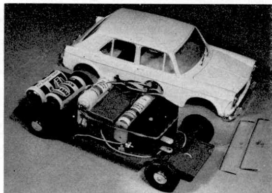
Shown above with the body-shell removed. The two piano wire parts at the right were used to secure the body to the chassis. This is more clearly seen in the heading photograph.
