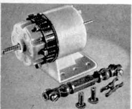
Power Drive 6-Ratio Gearbox with universal coupling Transmission ratios 3:1, 6:1, 12:1, 16:1, 32:1, 60:1. Can be coupled to any motor or other driving source that uses a 5/32" diameter spindle (Standard Meccano Rod size). £1.16.11.
