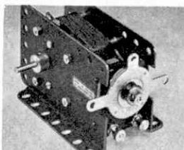
E15R Electric Motor 12/15 volt motor with built-in reversing switch. Will operate through transformer or give adequate power when run from suitable batteries. £3.9.11.
