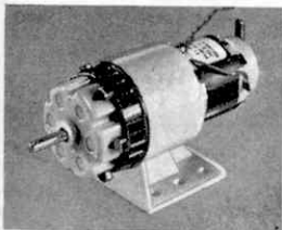
Power Drive Motor with 6-Ratio Gearbox Copper-graphite brushes have a life of more than 1,000 hours. Works from a 3-12 volts D.C. power supply. £2.15.11.
