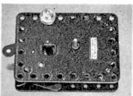
No. 1 Clockwork Motor Fitted with reversing mechanism – suitable for driving many of the larger models. £1.12.6.
