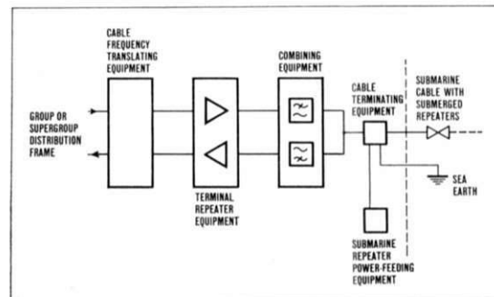
Above is a block diagram of typical submerged repeater. Below is a block diagram of typical terminal equipment for a submarine cable system.
