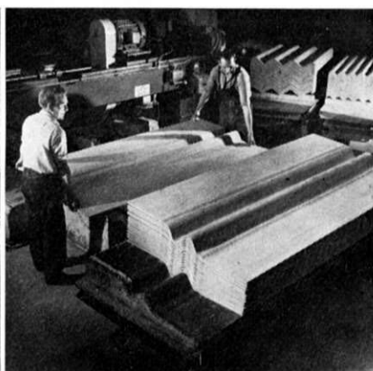
Left, shows two operatives using a high powered mechanical saw to trim "Turnall" Cavity Decking Sheets to the exact dimensions required.
