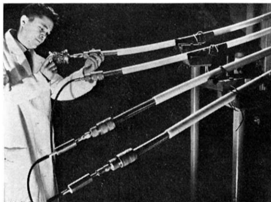
An engineer conducting transmission tests on completed lengths of a deep-water submarine cable.
