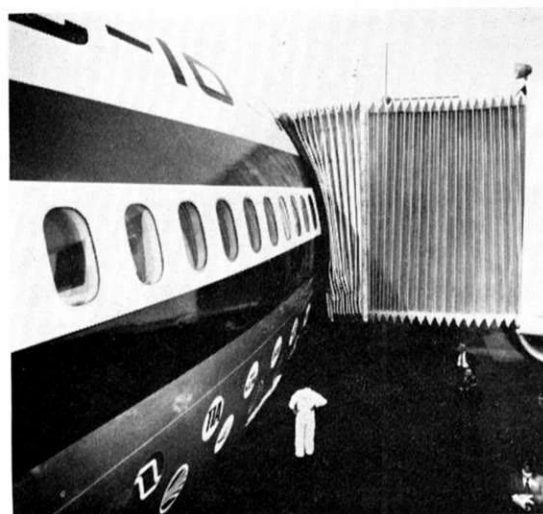
Above and below is the Plane-Mate joined to a McDonnell Douglas DC-10 of the American Airlines. Below right, a view inside a Plane-Mate.
