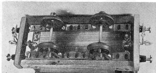
Above: Fig. 5, buffer beam and components of Primus Engineering Passenger Coach. Hooks and buffers have \frac{5}{32} " BSW thread as for Meccano. Below: Fig. 6, underside view of Coach showing Primus flanged wheels and trunnions. Note squared-off girder ends and narrow collar on axle.
