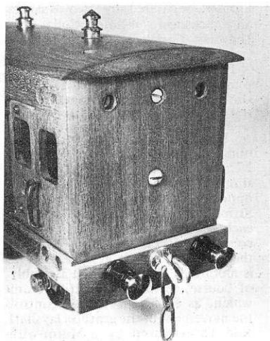
Above left: Fig. 3 showing close-up view of pre-formed wooden parts secured to inner metal framework by recessed bolts. Above right: Fig. 4, basic framework showing striking resemblance to Meccano parts.
