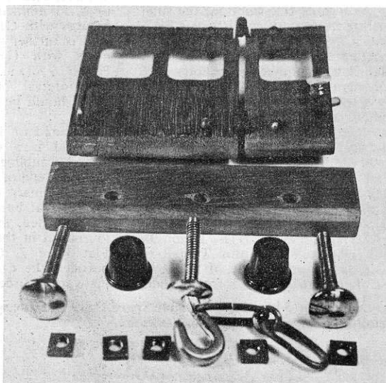
Above: Fig. 5, buffer beam and components of Primus Engineering Passenger Coach. Hooks and buffers have \frac{5}{32} " BSW thread as for Meccano. Below: Fig. 6, underside view of Coach showing Primus flanged wheels and trunnions. Note squared-off girder ends and narrow collar on axle.
