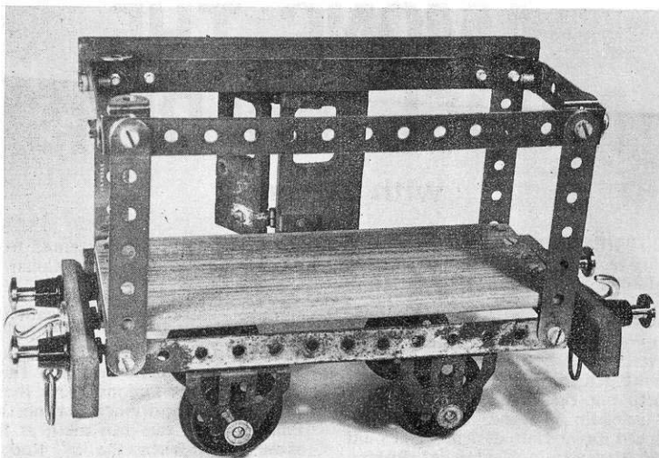
Above left: Fig. 3 showing close-up view of pre-formed wooden parts secured to inner metal framework by recessed bolts. Above right: Fig. 4, basic framework showing striking resemblance to Meccano parts.
