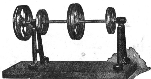
Transmission 4 poulies
